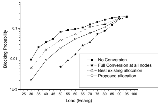
Figure 7. Performance of the proposed algorithm and the best existing allocation scheme.
