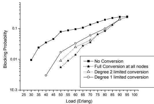
Figure 8. Limited range conversion at all nodes in the random generated network topology
